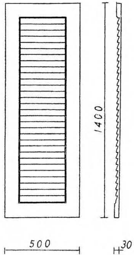
Ante-HLS 1400-500
